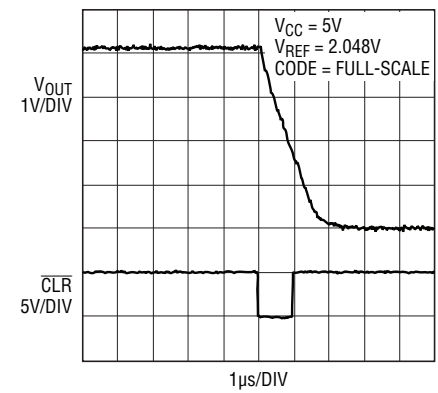
Hardware \overline{\text{CLR}} to Zero-Scale
