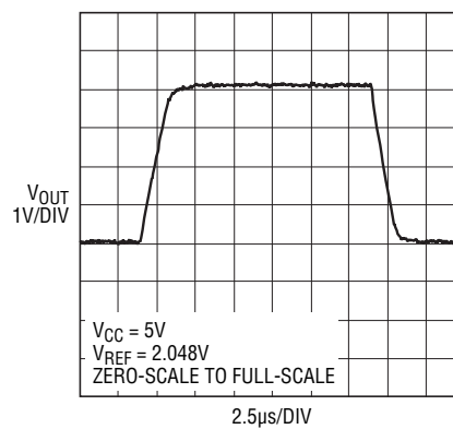
Large-Signal Response
